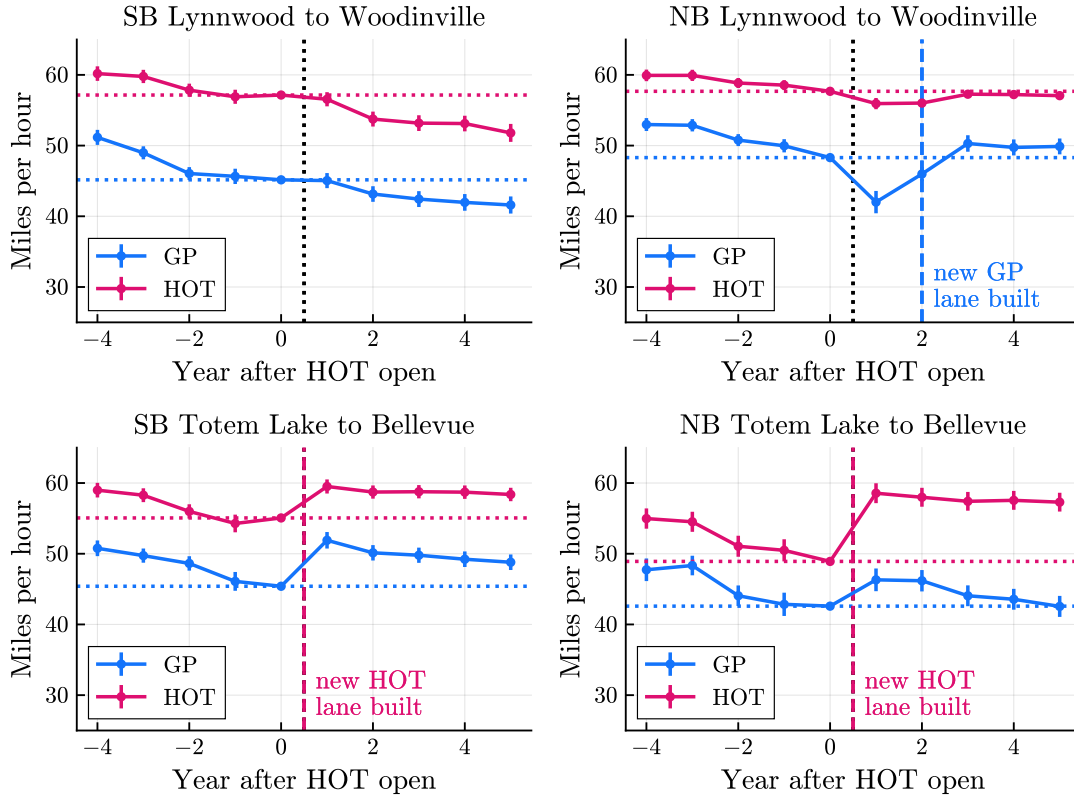
Figure C.22: Long-run changes in speed by road segment
