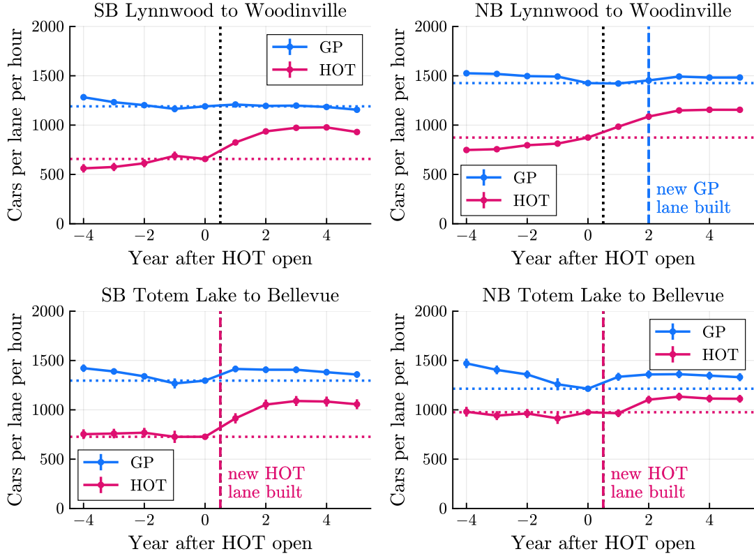
Figure C.23: Long-run changes in throughput by road segment
